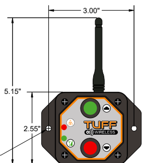
P/N: 3A577CA RECEIVER, 3 OUTPUTS
