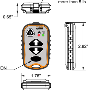
P/N: 3A577BA TRANSMITTER, MICRO, 3 BUTTON
