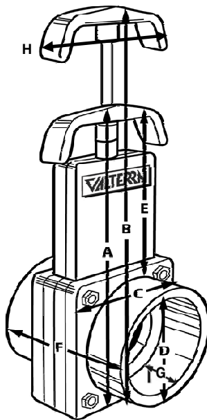
6" Valterra Gate Valve with Extension Rod
